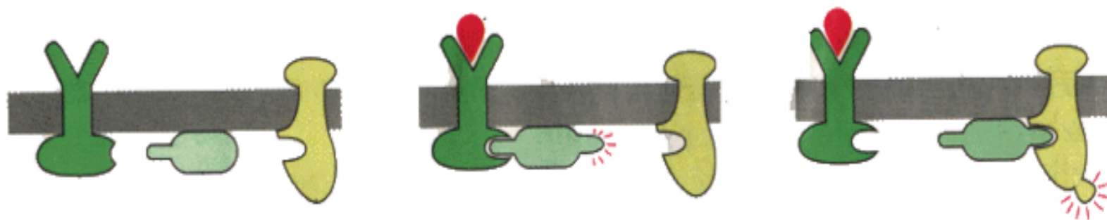
G-protein linked receptor
