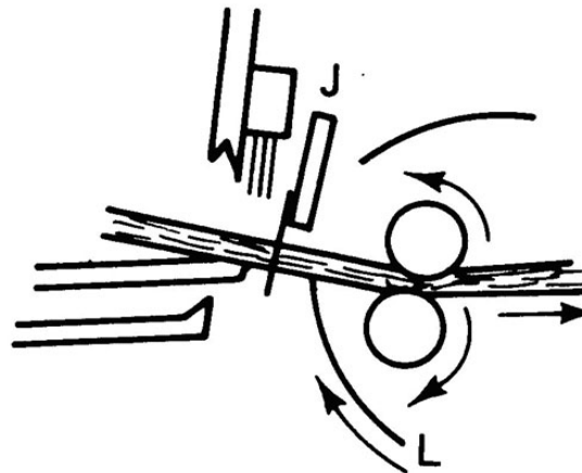
Figure 7.10 Combing cycle: counter-sword raised. Source: Wood, 2006.
