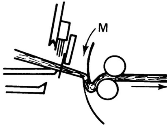
Figure 7.11 Combing cycle: Top sword lowered (for very long fibres).
