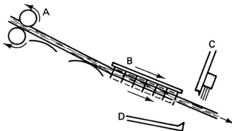
Figure 7.6 Combing cycle: feeding. Source: Wood, 2006.
