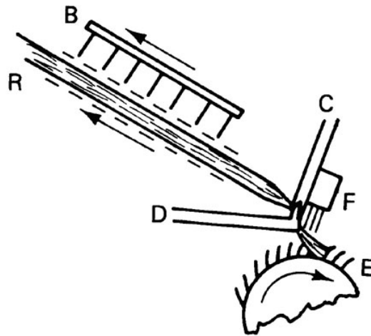
Figure 7.7 Combing cycle: initial combing. Source: Wood, 2006.
