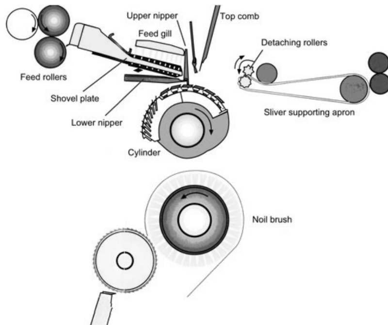
Figure 7.5 Rectilinear comb – side elevation. Adapted from: NCS Schlumberger.
