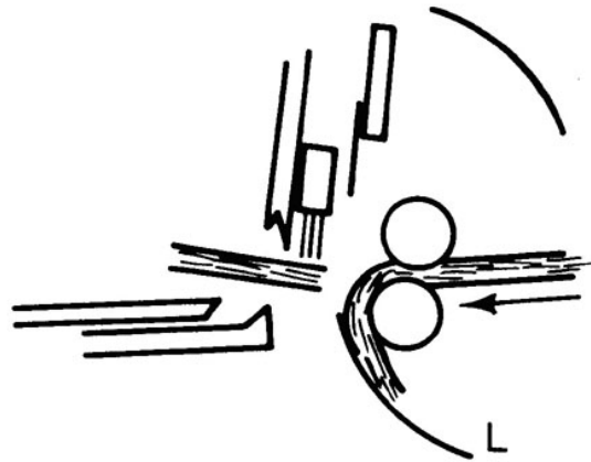
Figure 7.13 Combing cycle: overlapping of tufts about to commence. Source: Wood, 2006.
