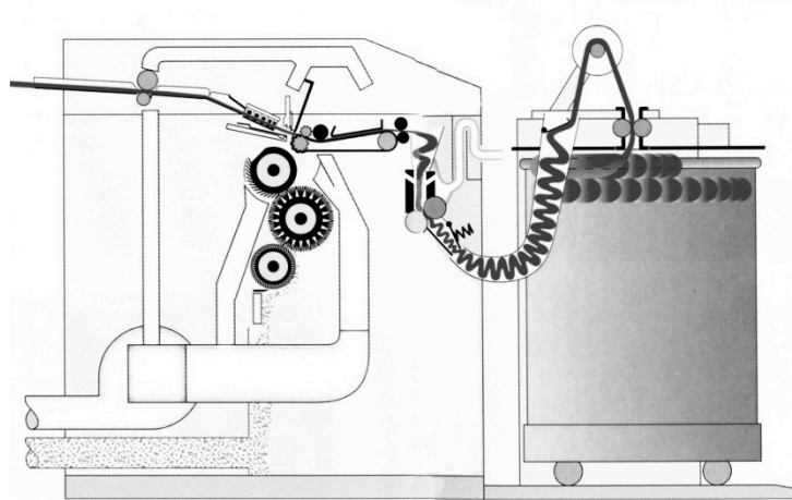
Figure 7.3 Cross-section view of a rectilinear combing machine. Source: NCS Schlumberger.
