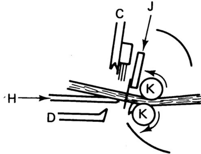
Figure 7.9 Combing cycle: final combing and drawing off. Source: Wood, 2006.
