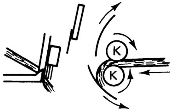
Figure 7.12 Combing cycle: recoil of the detaching rollers. Source: Wood, 2006.
