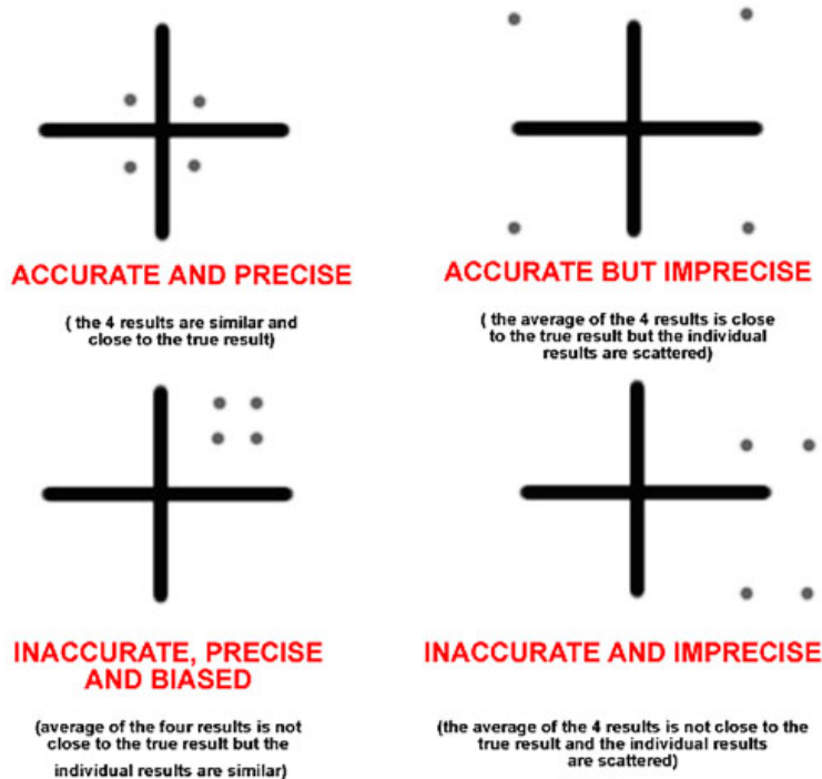
Figure 5.2 This illustration demonstrates the difference between ACCURACY , PRECISION and BIAS . The “true” result is defined as the point where the two lines intersect and the 4 dots represent the results of 4 separate measurements. Source: Douglas (2000).
