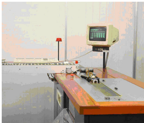
Figure 10.4 An automatic tester for length and strength (ATLAS).
