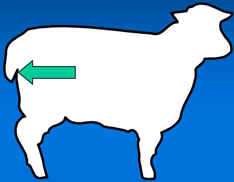
Along-staple variation
