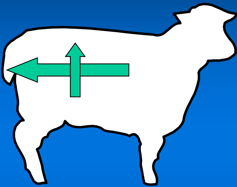
Standard deviation
