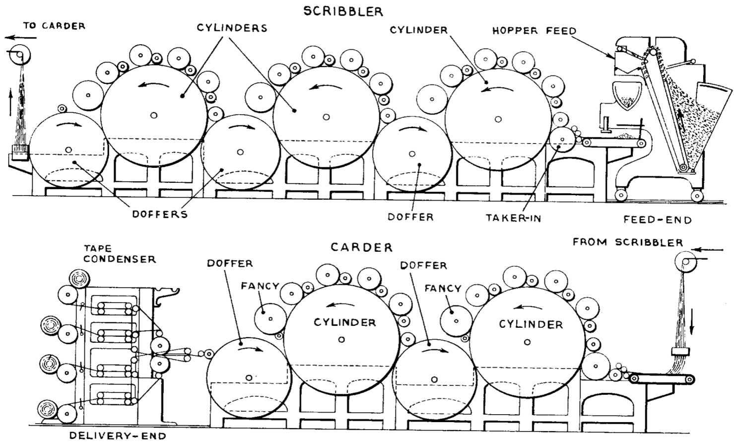
FIG. 17. YORKSHIRE CARDING SET
